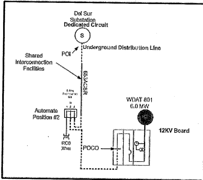
Figure 2-2: Proposed Single Line Diagram
