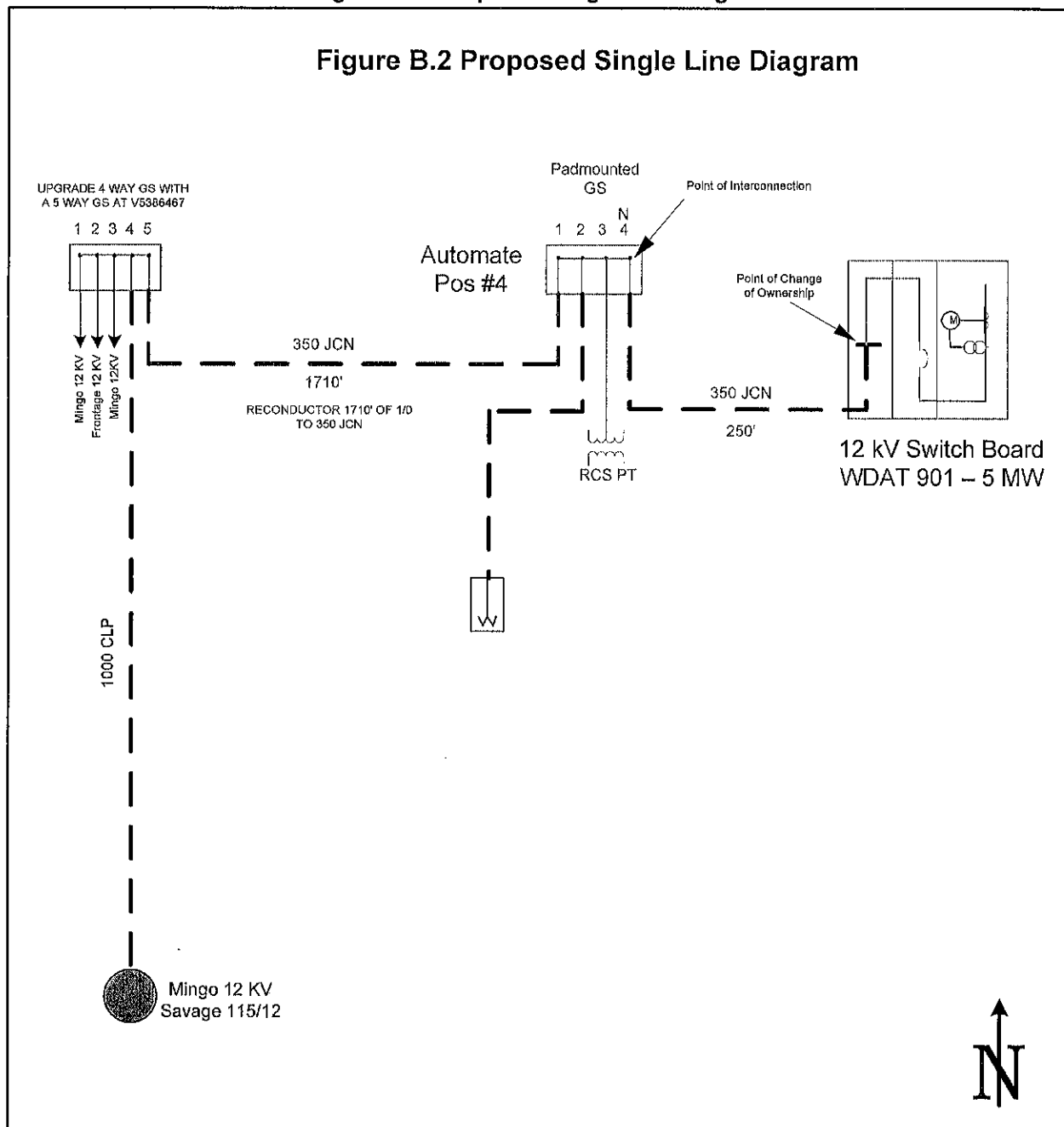
Figure B.2: Proposed Single Line Diagram
