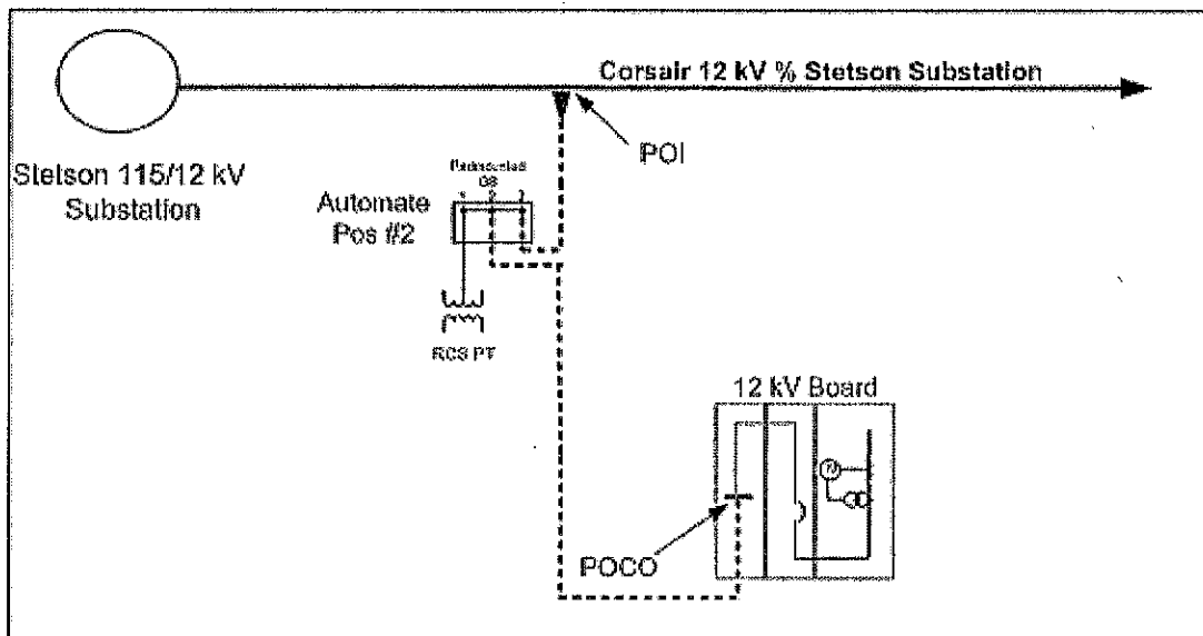
Figure 2-2: Proposed Single Line Diagram
