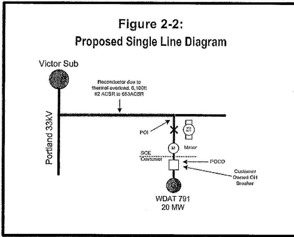
Figure 2-2: Proposed Single Line Diagram
